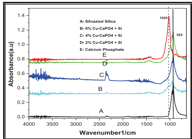
Fig.2: Ftir Analysis of Salinized Silica, Dental Composite, 2,4,6% Copper Doped Calcium Phosphate in Dental Composite
